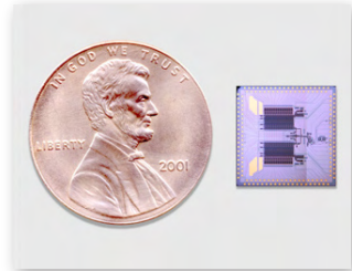
All-Digital Receiver on a One-Centimeter Superconducting Niobium Chip Image courtesy of Hypra, Inc.
